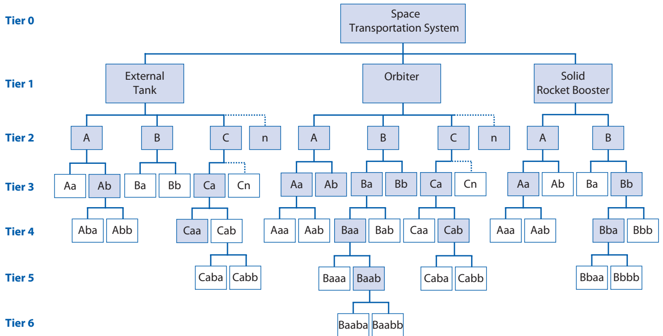
Figure 2.3-6 Product hierarchy: complete pass through system design processes side of the SE engine
